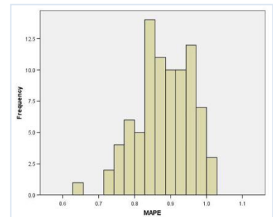
[평균절대비율오차]
